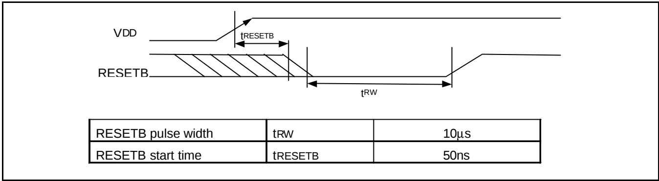
Figure 14. RESET Timing
