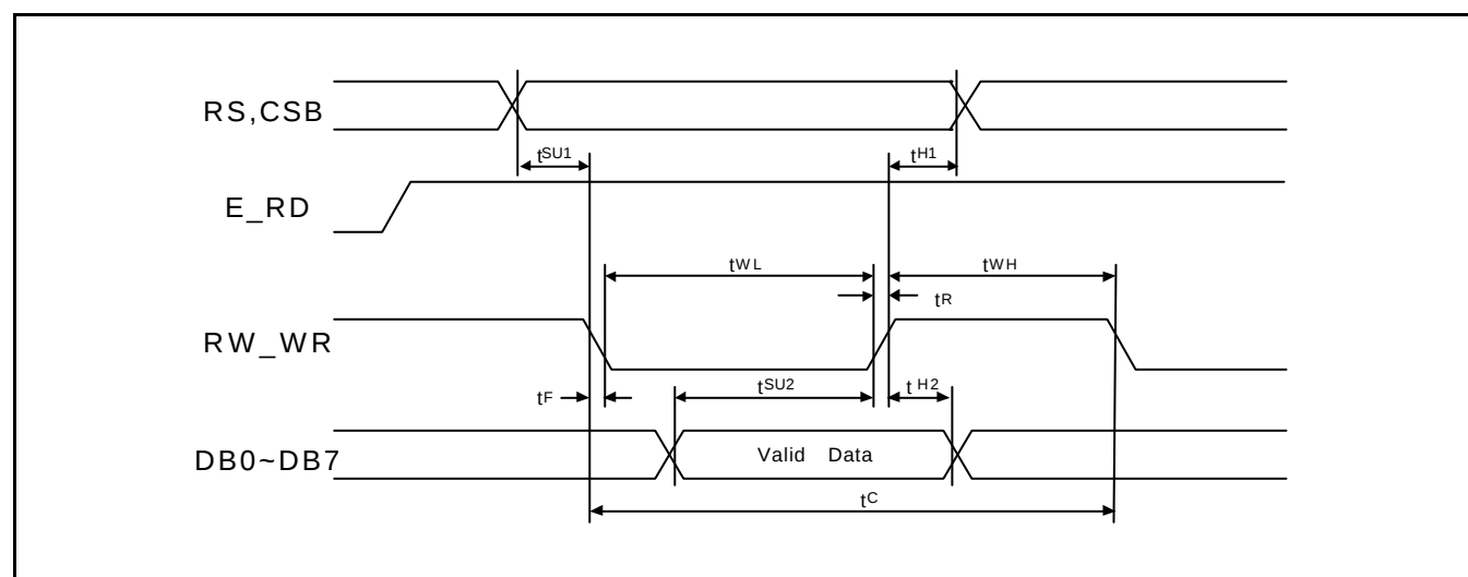
Figure 29. Write Timing Diagram (80-series)
