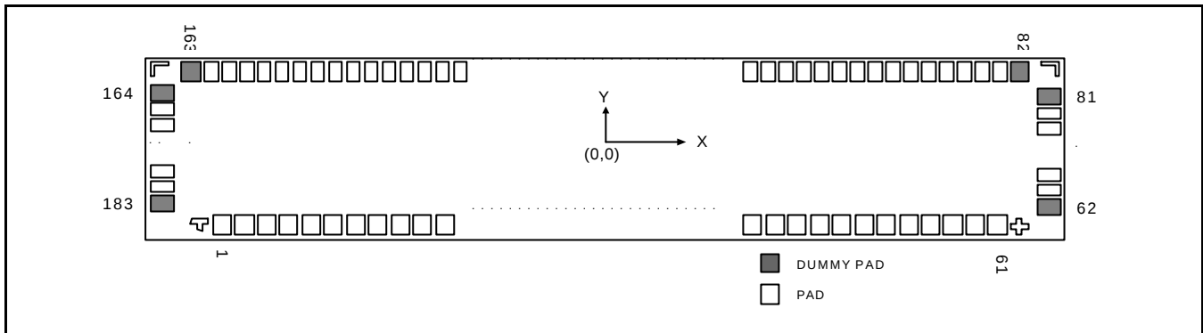
Figure 2. Pad Configuration
