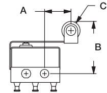
FIG. 4 Leaf Roller
