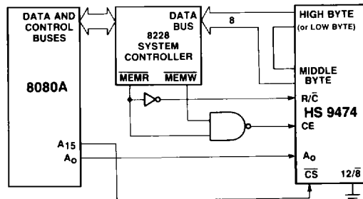
Figure 5. Interfacing the HS 9474 and 8080A μP
