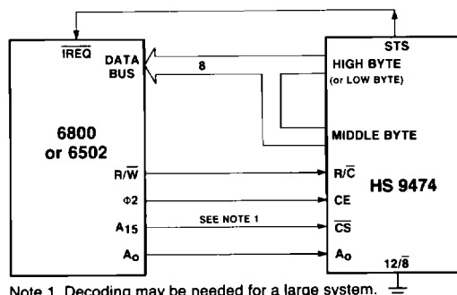
Figure 4. Interfacing the HS 9474 and a 6800 μP
