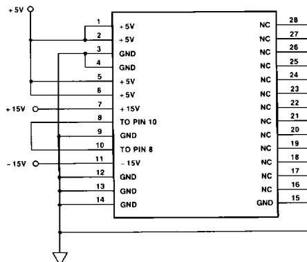
Figure 10. Burn-In Schematic
