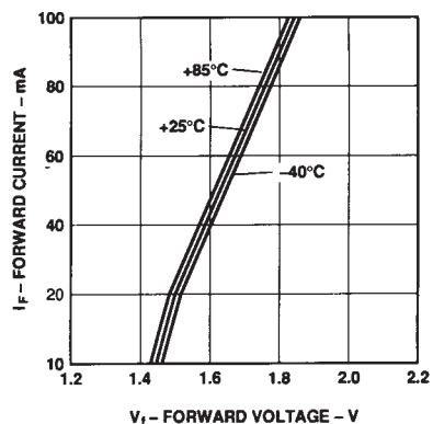
Figure 9. Forward Voltage and Current Characteristics.
