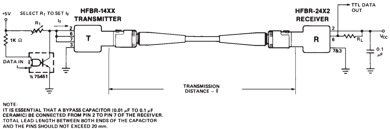
Figure 2. Typical Circuit Configuration.
