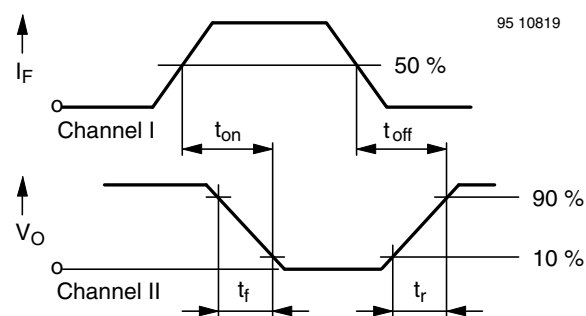
Figure 2. Pulse Diagram
