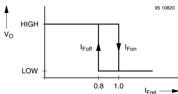
Figure 3. Hysteresis
