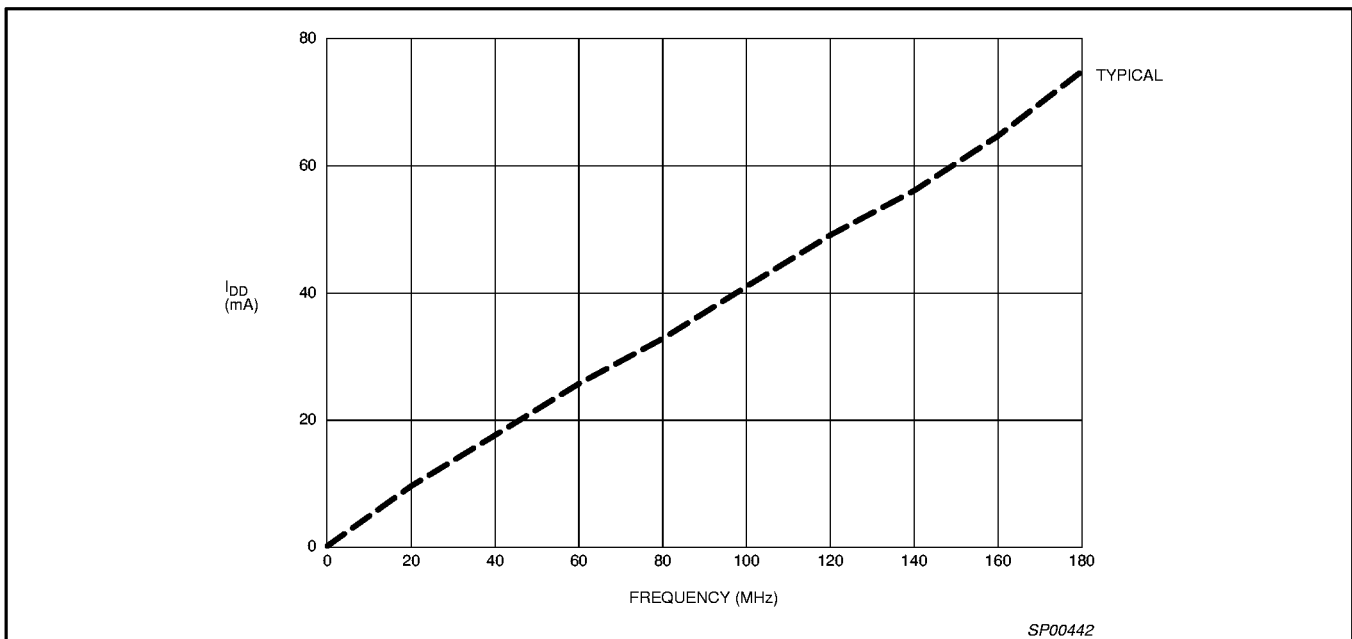
Figure 5. I_{DD} vs. Frequency @ V_{DD} = 5.0V , 25^{\circ}C
