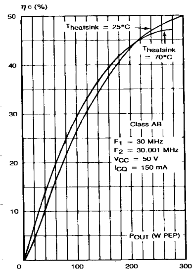
COLLECTOR EFFICIENCY vs POWER OUTPUT PEP
