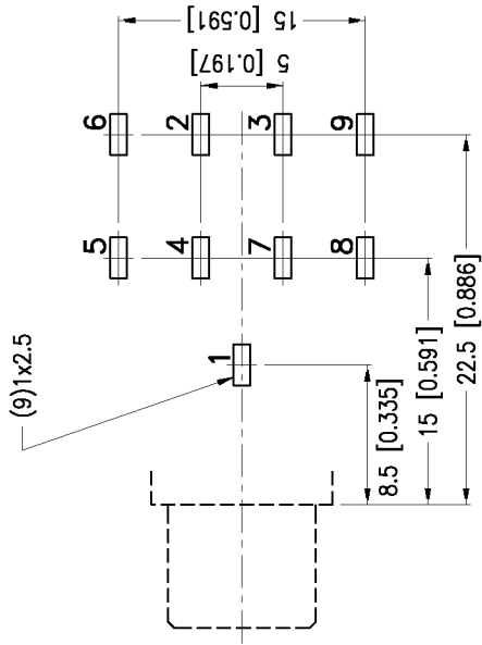
HOLE LAYOUT (BOTTOM VIEW)
