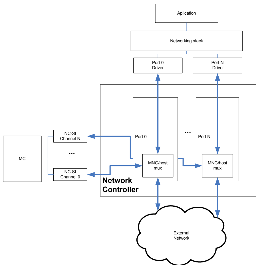
Figure 11-3. OS-to-BMC Diagram
