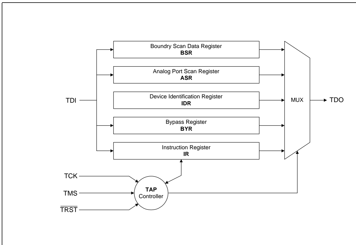
Figure 12. JTAG Architecture
