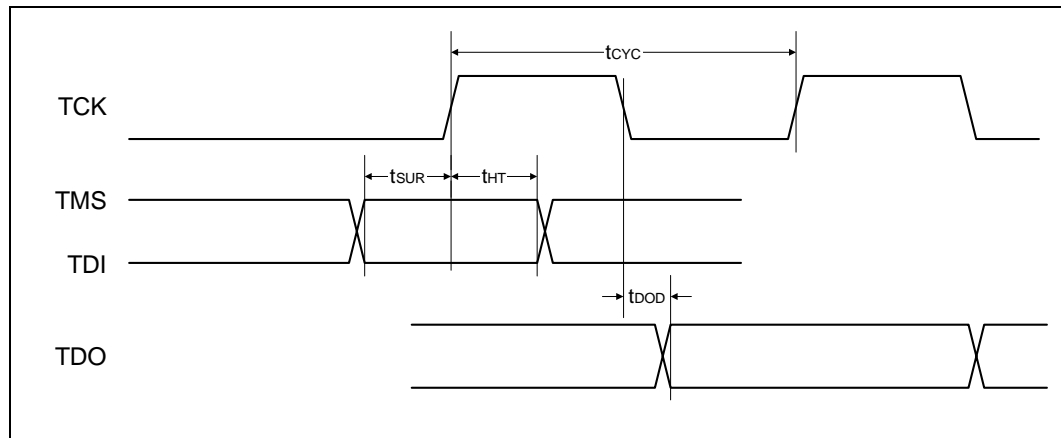
Figure 17. JTAG Timing
