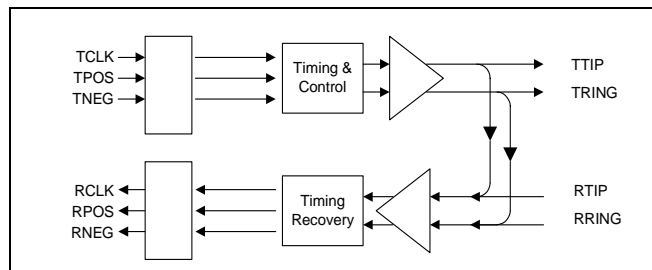
Figure 8. Analog Loopback
