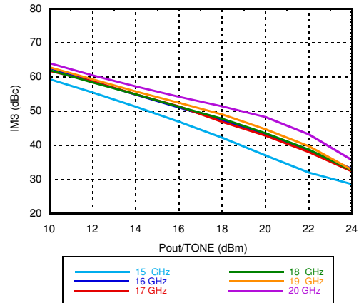
Output IM3 @ V_{dd} = +5.5V , 1000mA
