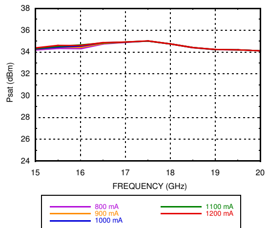
Psat vs. Supply Current
