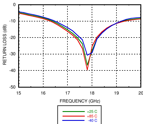
Input Return Loss vs. Temperature
