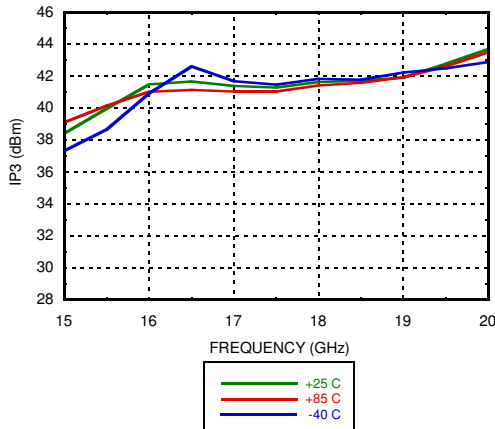
Output IP3 vs. Temperature, Pout/tone = +20 dBm
