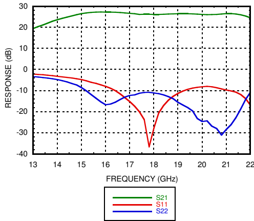
Gain & Return Loss
