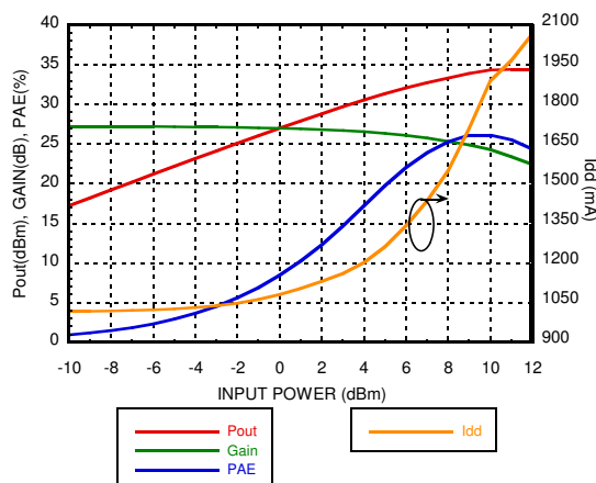
Power Compression @ 17.5 GHz
