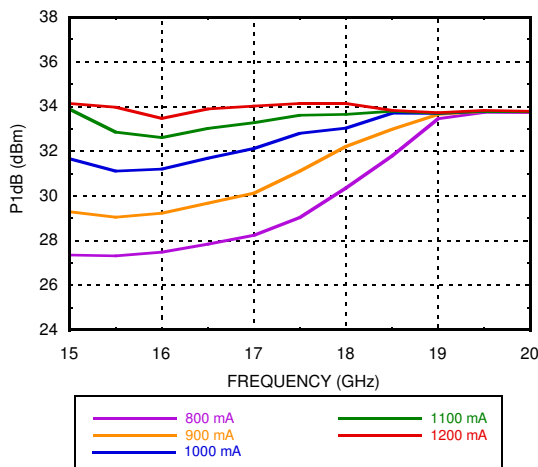
P1dB vs. Supply Current
