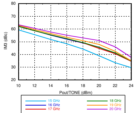
Output IM3 @ Vdd = +6V
