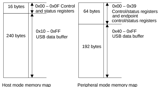
Figure 2-2. Memory Map
