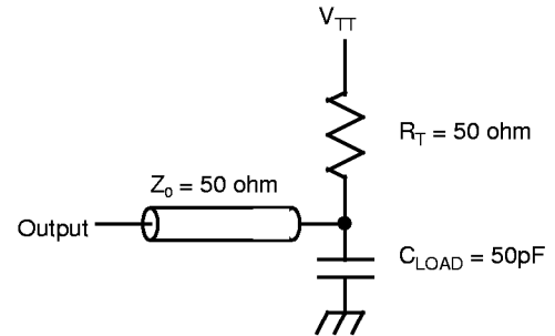
AC Output Load Circuit
