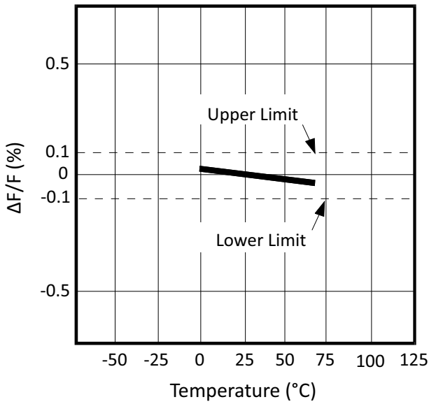
Figure 4: % \Delta Freq. vs. Temperature (SWR200C)
