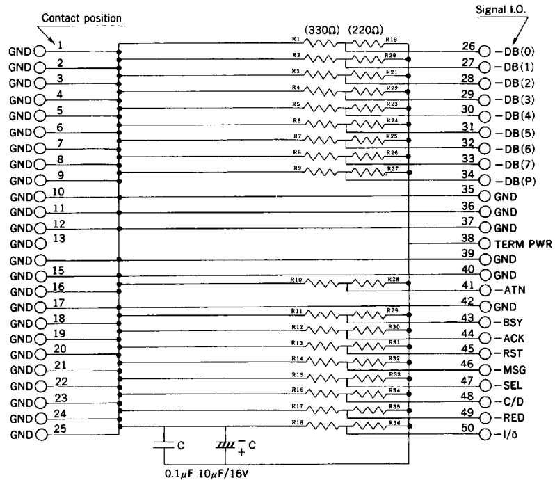
Standard circuit #2 (with capacitor)
