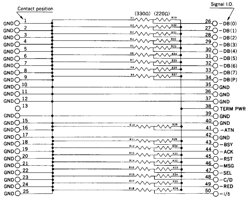
Standard circuit #1 (less capacitor)
