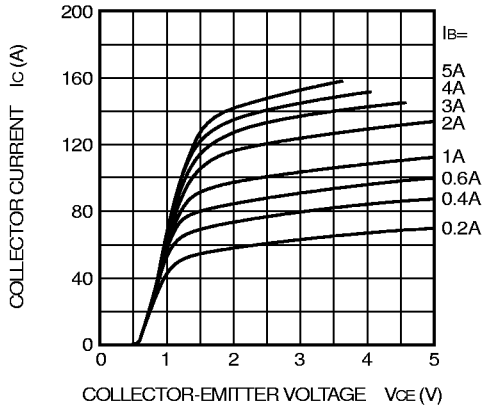
COMMON EMITTER OUTPUT CHARACTERISTICS (TYPICAL)
