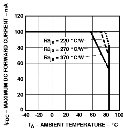
Figure 6. Maximum DC Forward Current vs. Ambient Temperature. Derated Based on T_{JMAX} = 110^{\circ}C .
