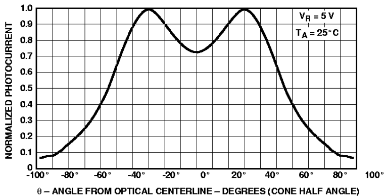
Figure 18. Relative Radiant Intensity vs. Angular Displacement. HSDL-5400.
