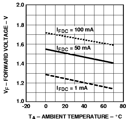
Figure 3. Forward Voltage vs Ambient Temperature.
