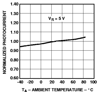
Figure 13. Relative Reverse Light Current vs. Ambient Temperature.
