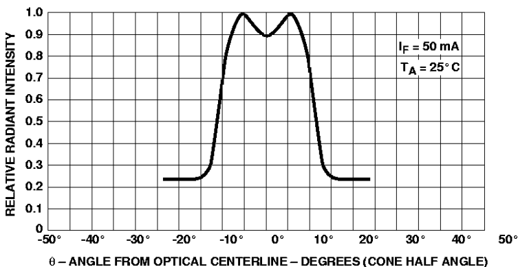
Figure 10. Relative Radiant Intensity vs. Angular Displacement HSDL-4420.
