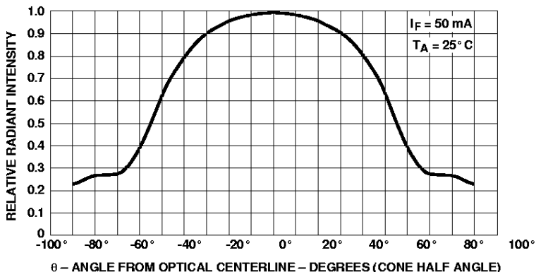
Figure 9. Relative Radiant Intensity vs. Angular Displacement HSDL-4400.
