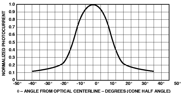
Figure 19. Relative Radiant Intensity vs. Angular Displacement. HSDL-5420.
