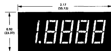
CASE DEPTH LED and LCD BACKLIT: 0.56 in. (14.22mm) LCD: 0.43 in. (10.92mm) DIGIT HEIGHT LED: 0.52 in. (13.2mm) LCD: 0.40 in. (10.2mm)
