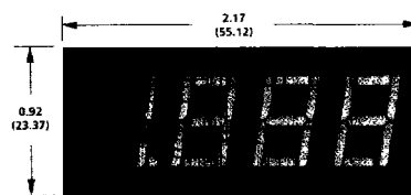
CASE DEPTH LED and LCD BACKLIT: 0.56 in. (14.22mm) LCD: 0.43 in. (10.92mm) DIGIT HEIGHT LED: 0.56 in. (14.2mm) LCD: 0.40 in. (10.2mm)
