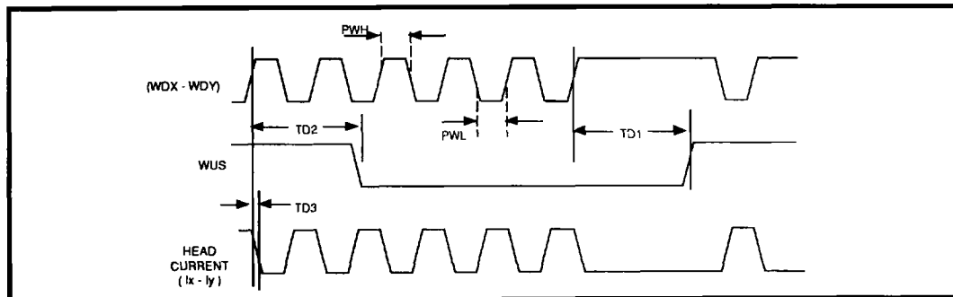
FIGURE 1: 32R2502R Write Mode Timing Diagram
