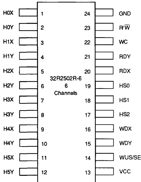
24-Lead SOV, SOL
