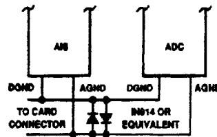
Figure 11. Ground-Fault Protection Diodes
