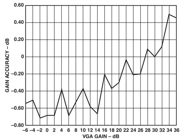
TPC 12. PGA Gain Error vs. Gain
