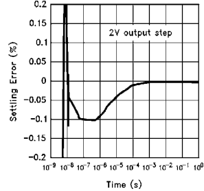
Long-Term Settling Time
