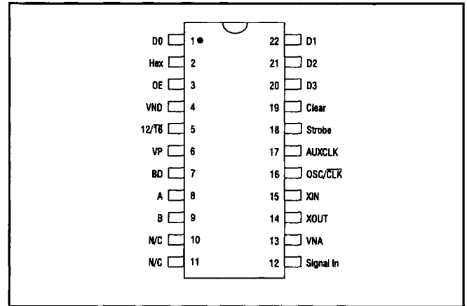
Figure 1 Pin Diagram
