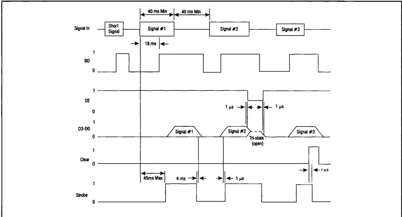
Figure 3 Timing Diagram
