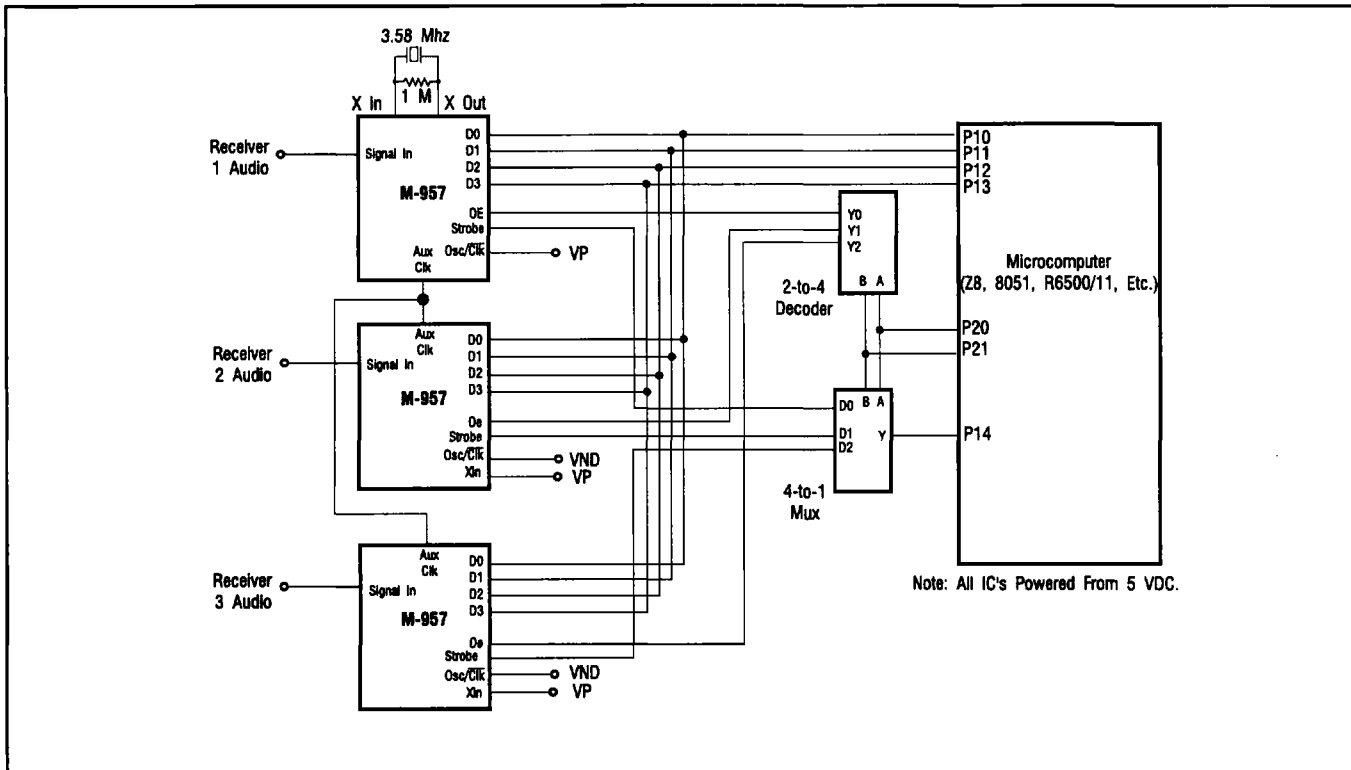
Figure 5 Multiple Receiver/Microprocessor Interface
