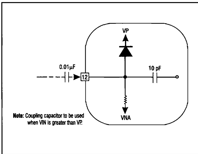
Figure 8 Input Signal Configuration
