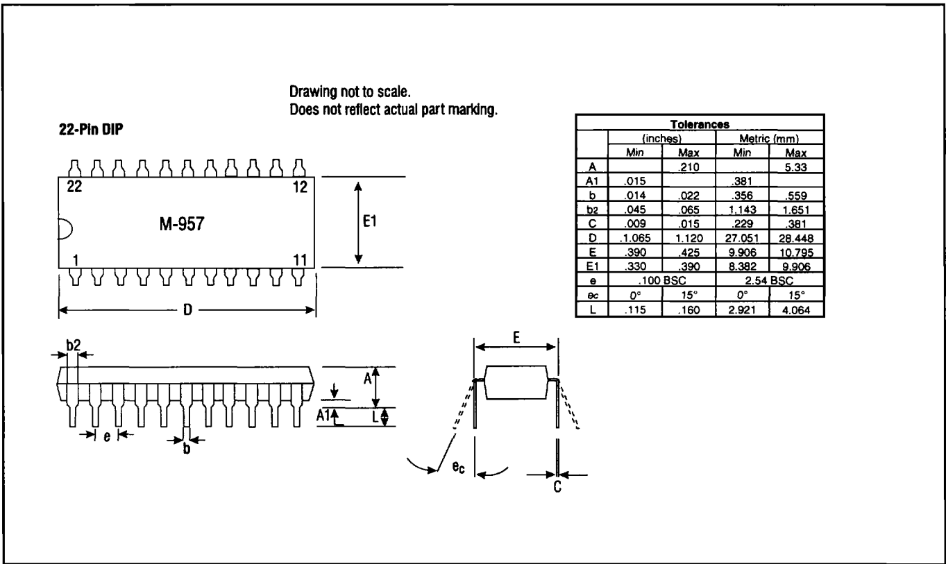
Figure 7 Package Dimensions
