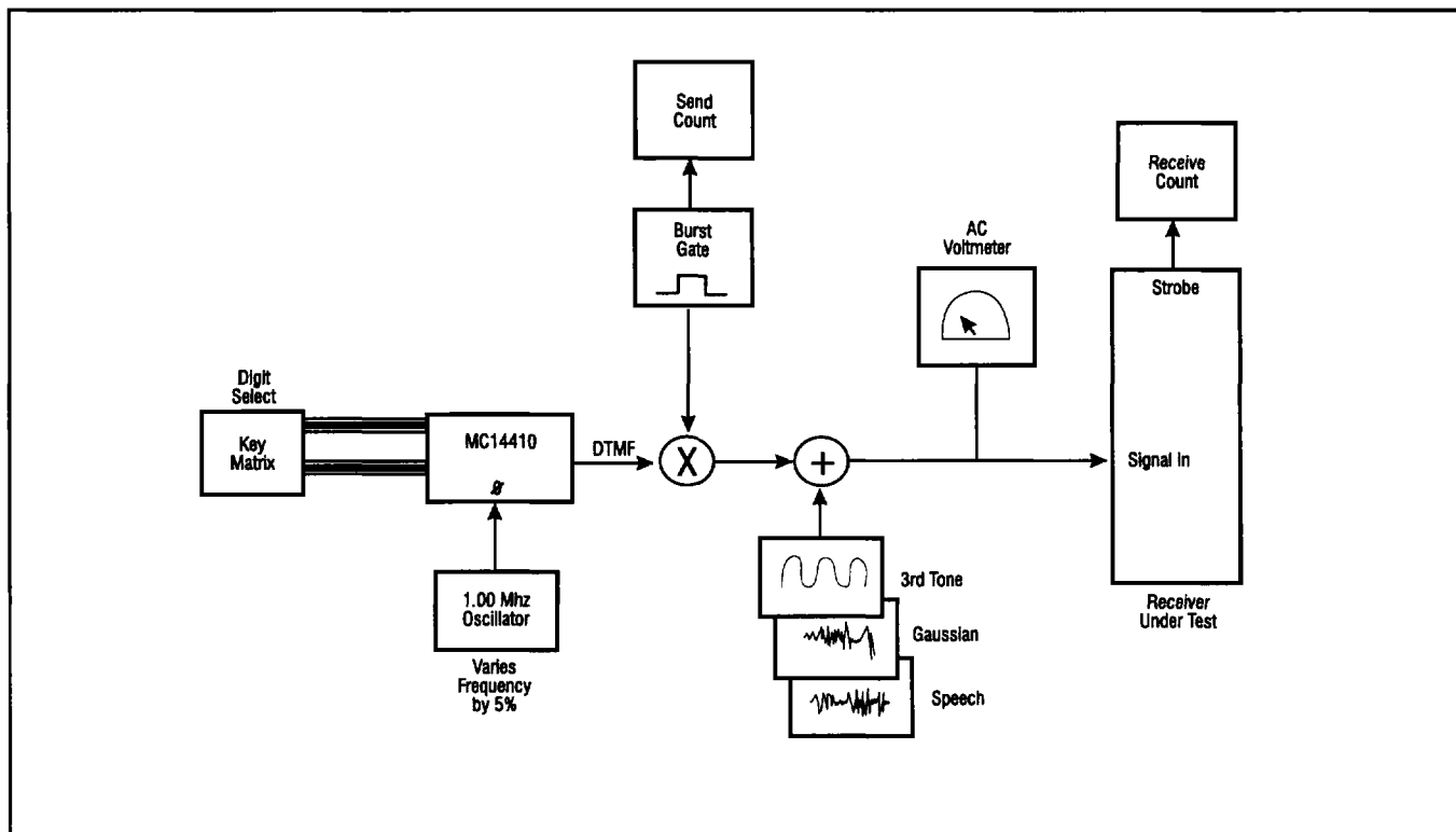
Figure 6 Test Circuit
