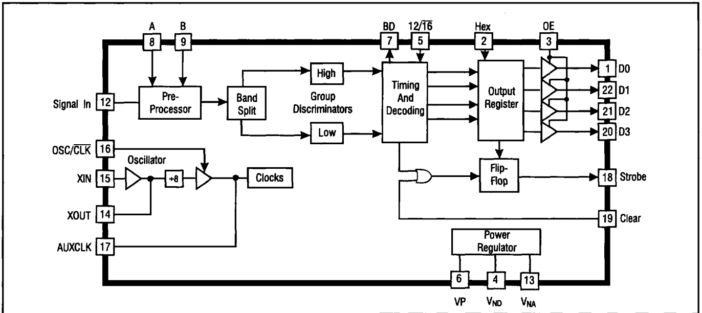
Figure 2 Block Diagram
