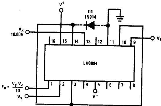
FIGURE 2a. LH0094 Used to Multiply (No External Adjustment)
