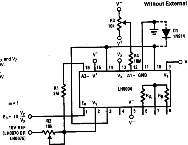
FIGURE 5. Precision Divider (0.05% Typ)
