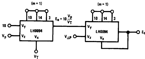
FIGURE 12. Vector Magnitude Function
