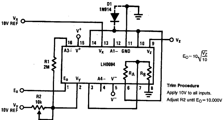
FIGURE 9. Precision Square Rooter (0.15% Typ)
