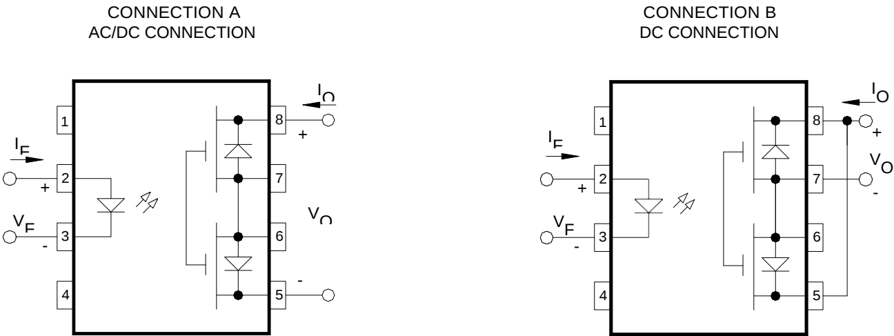
Figure 1 - Terminal Connections
