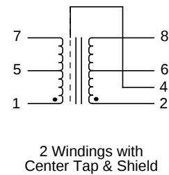
Schematic
