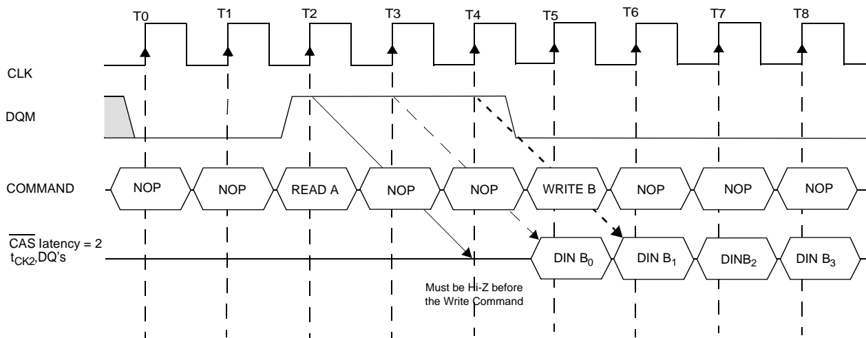
Read to Write interval (Burst Length = 4, \overline{\text{CAS}} Latency = 2)
