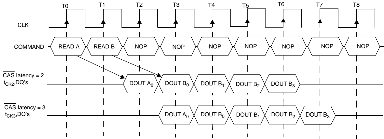
Read Interrupted by a Read (Burst Length = 4, CAS Latency = 2, 3)
