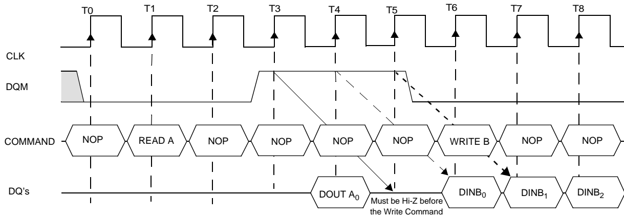
Read to Write interval (Burst Length = 4, \overline{\text{CAS}} Latency = 3)
