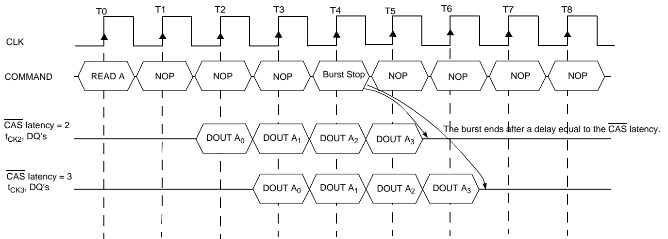
Termination of a Burst Read Operation (Burst Length > 4, \overline{\text{CAS}} Latency = 2, 3)
