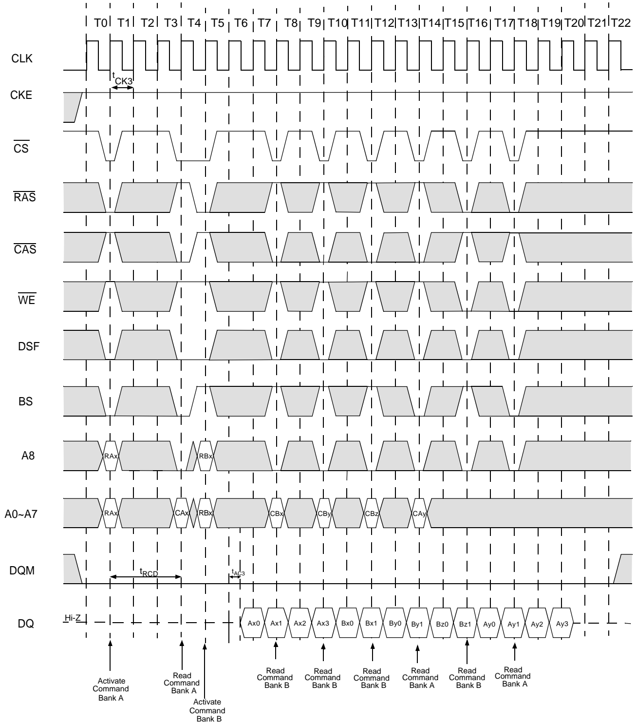
Figure 14.2 Interleaving Column Read Cycle (Burst Length = 4, CAS Latency = 3)
