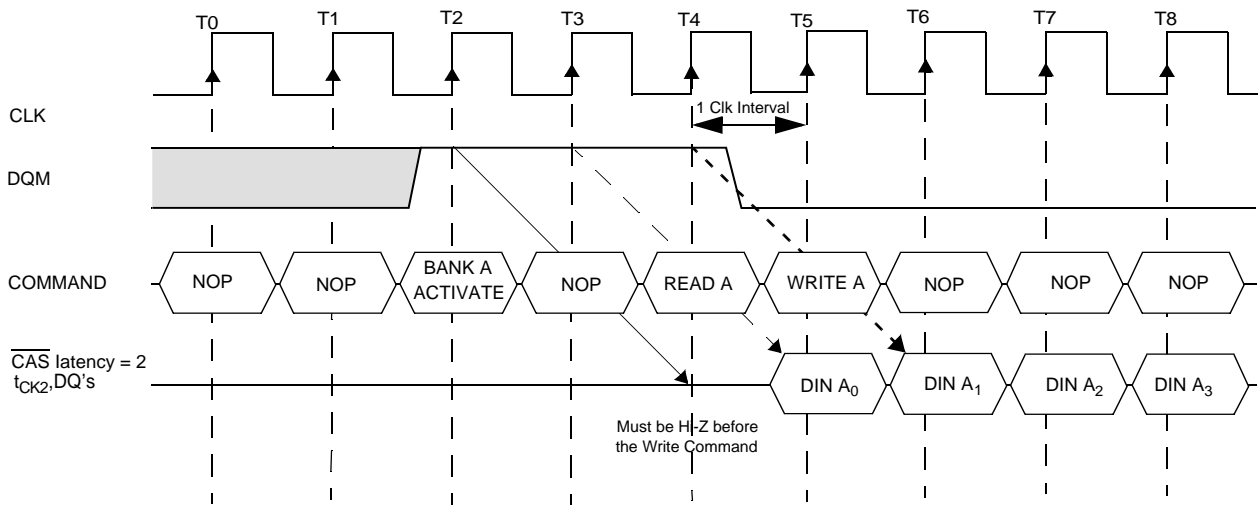
Read to Write interval (Burst Length = 4, \overline{\text{CAS}} Latency = 2)
