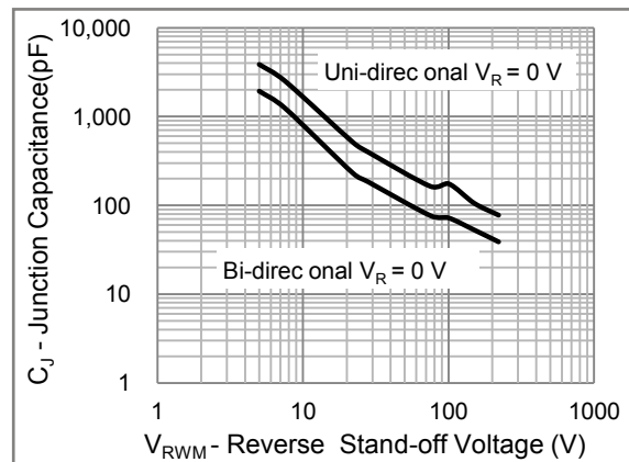
Fig.4 Typical Capacitance
