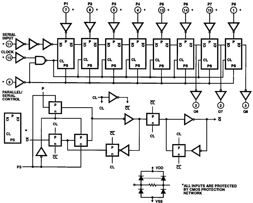
FIGURE 2. CD4021BMS LOGIC DIAGRAM
