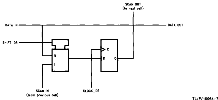
Scan Cell TYPE2
