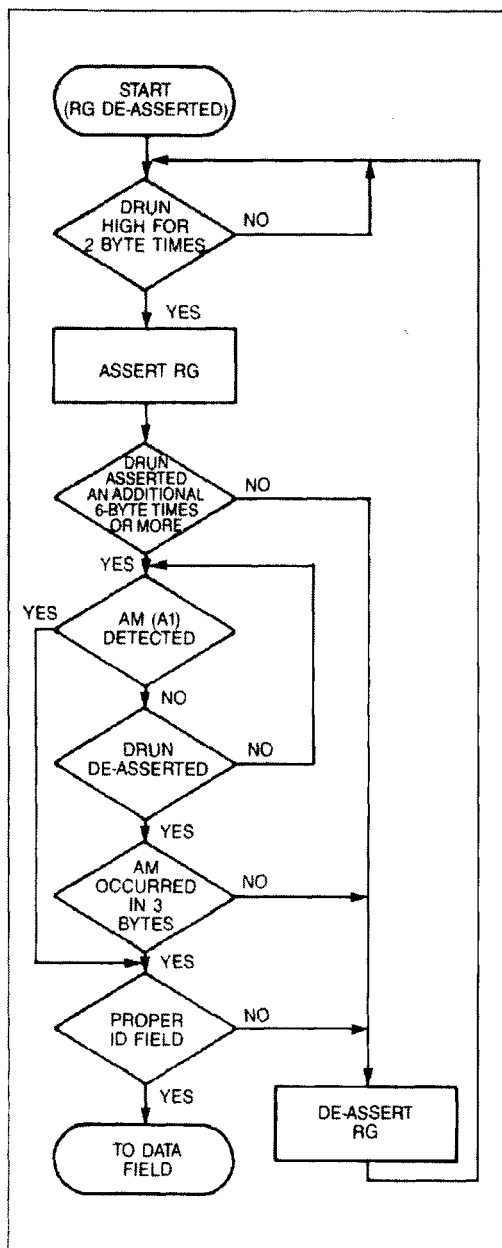
FIGURE 4. PLL CONTROL (ID FIELD)
