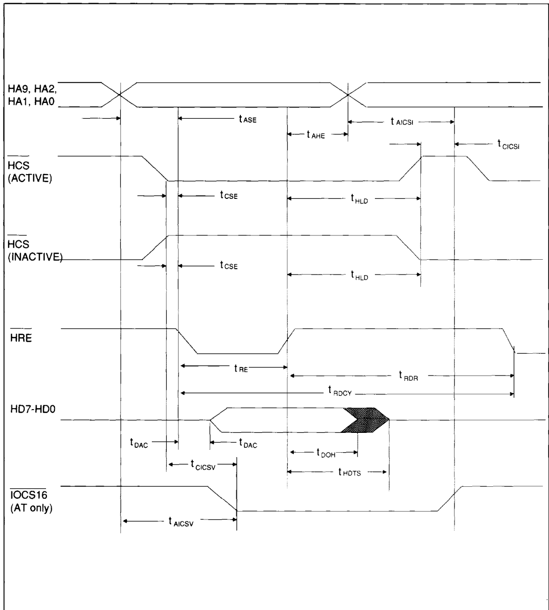
FIGURE 9. AT/XT HOST PROGRAMMED I/O READ TIMING
