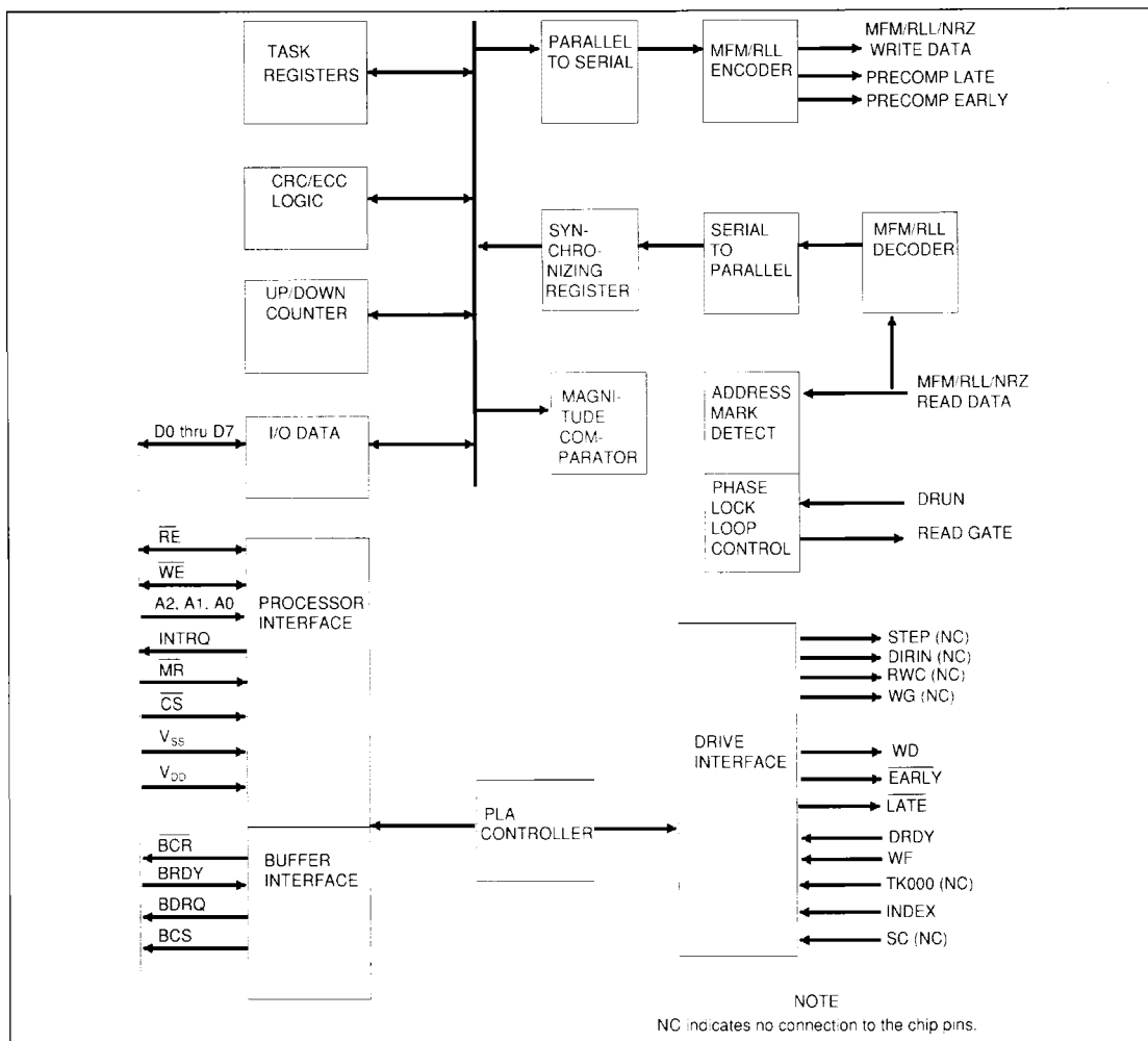
FIGURE 3. DRIVE CONTROLLER BLOCK DIAGRAM
