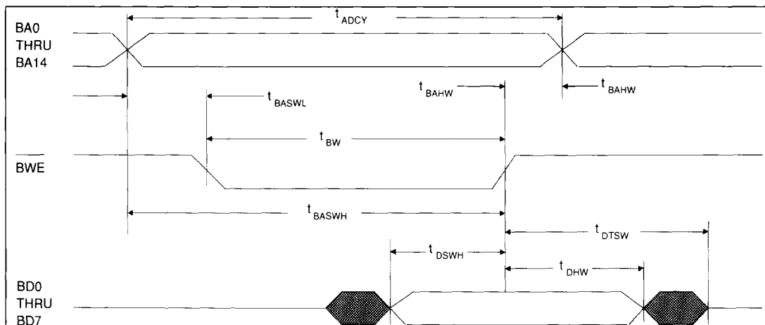
FIGURE 16. BUFFER RAM WRITE TIMING (INTERNAL OSCILLATOR)
