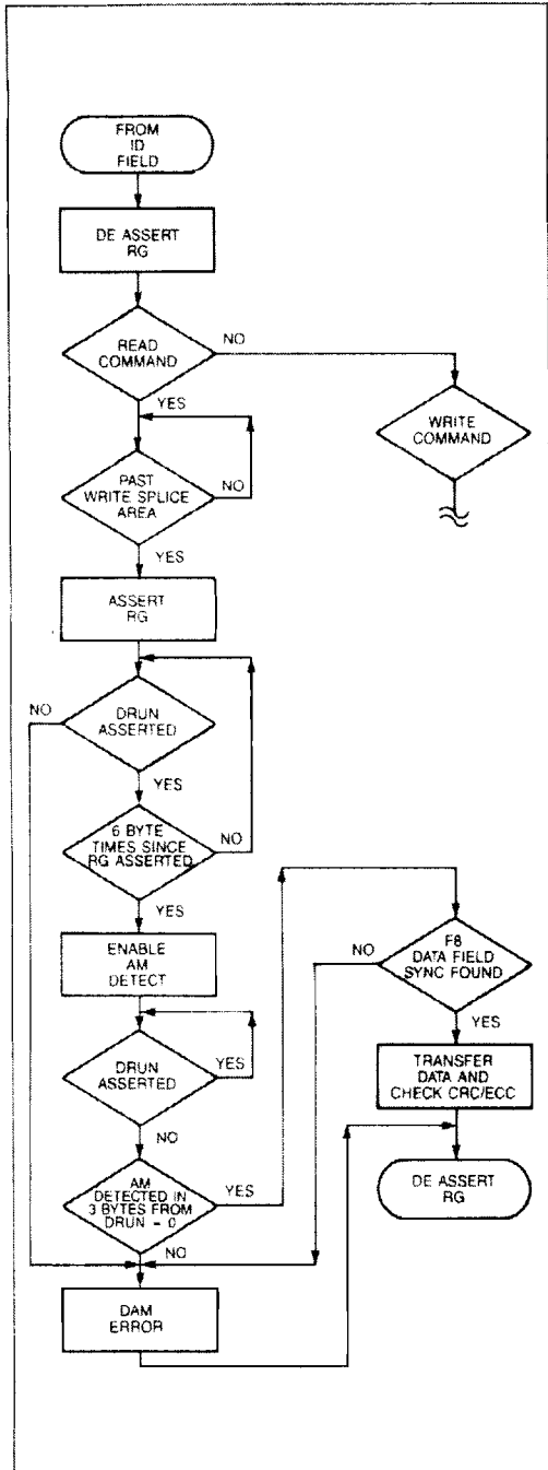
FIGURE 5. PLL CONTROL (DATA FIELD)
