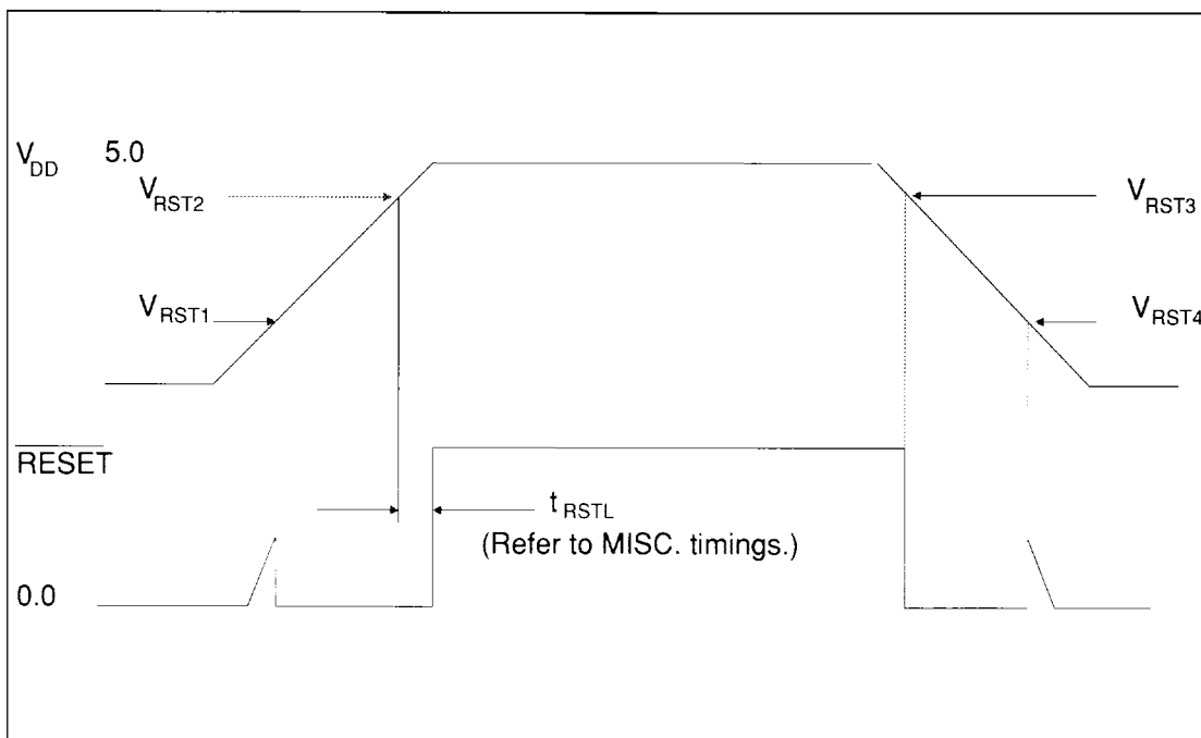
FIGURE 6. POWER QUALIFIED RESET VOLTAGE THRESHOLD
