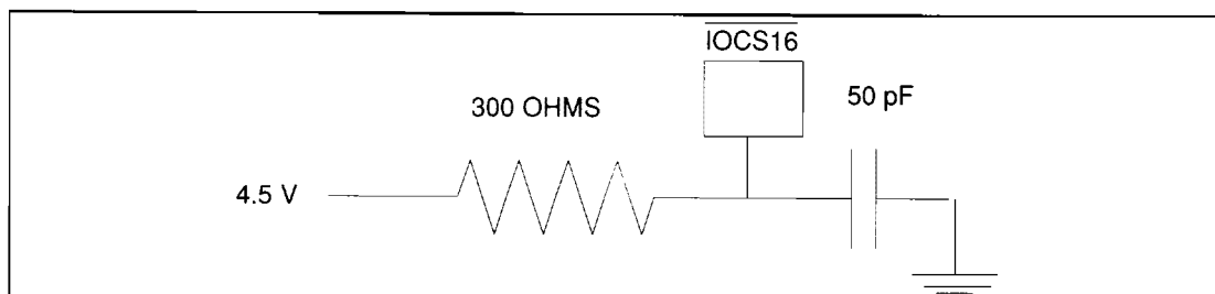
FIGURE 8. TEST CIRCUIT 1
