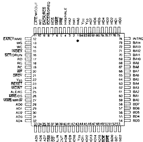
FIGURE 1. 84-PIN PLCC OR PQFP
