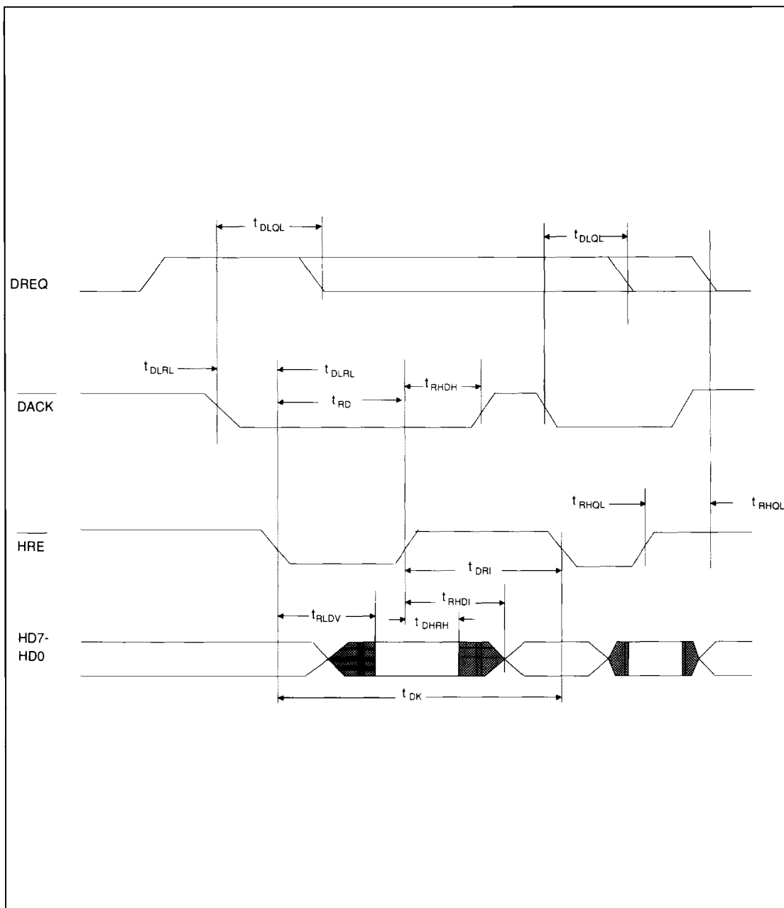
FIGURE 11. AT/XT HOST DMA READ TIMING
