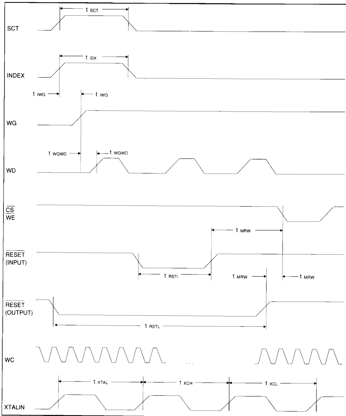
FIGURE 28. MISCELLANEOUS TIMING
