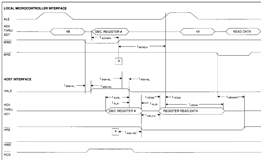
FIGURE 13. SLAVE HOST READ TIMING
