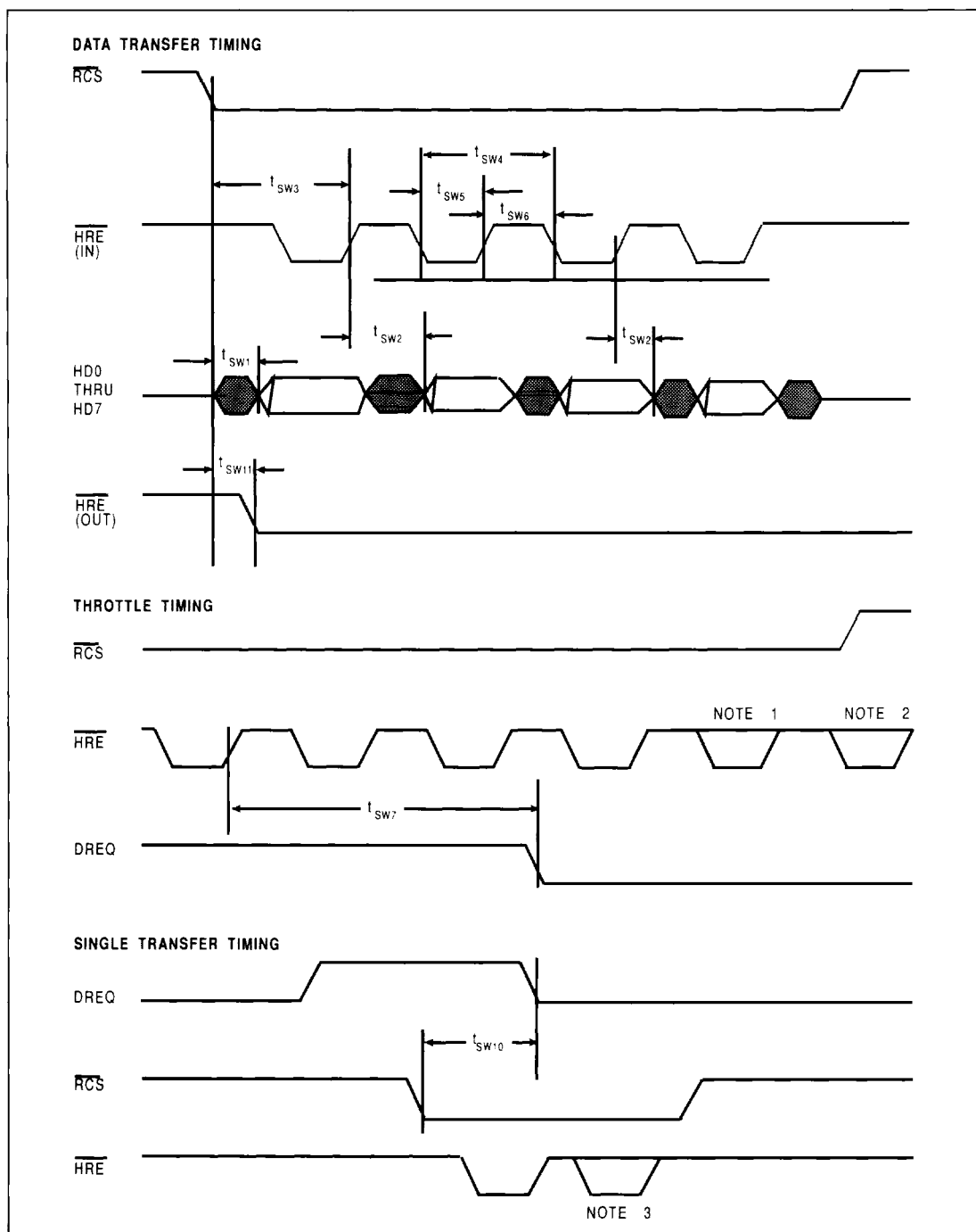
FIGURE 15. SLAVE HOST DMA READ TIMING
