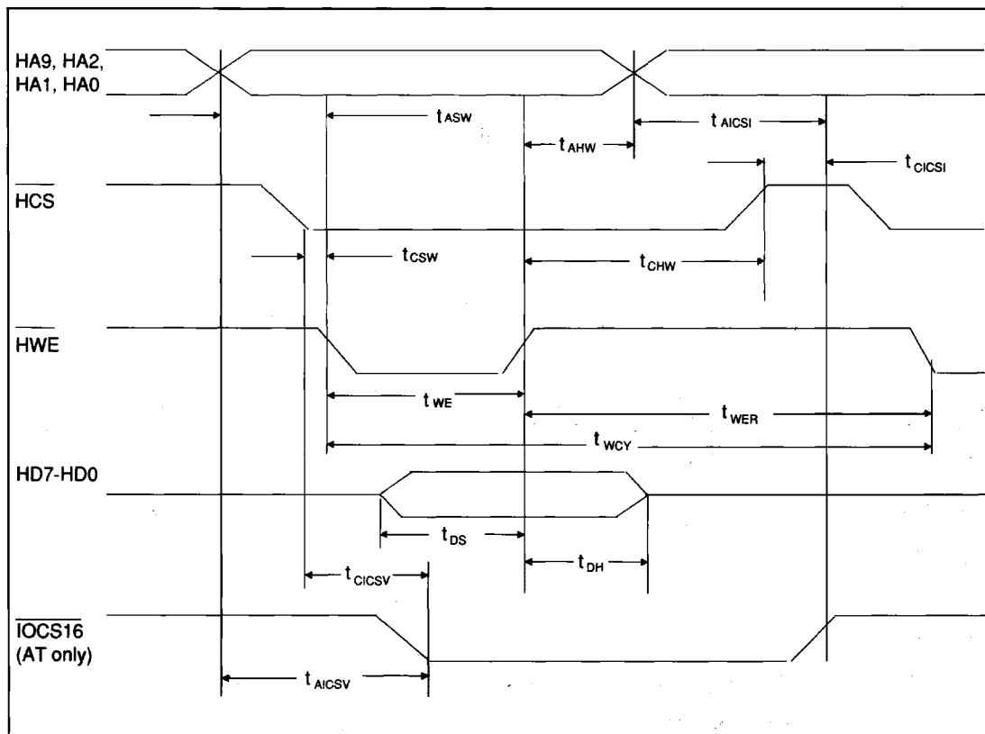
FIGURE 7. AT/XT HOST PROGRAMMED I/O WRITE TIMING
