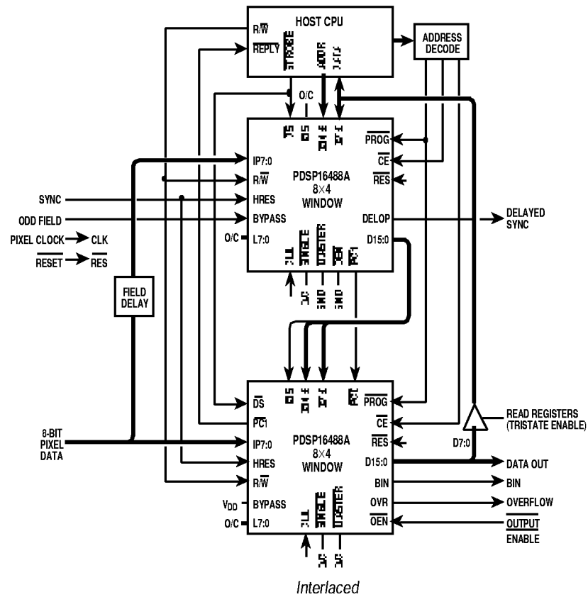
Fig. 14 8-bit dual device systems
