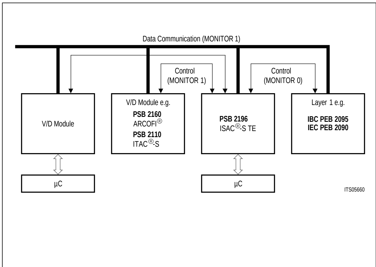
Figure 17 Examples of MONITOR Channel Applications
