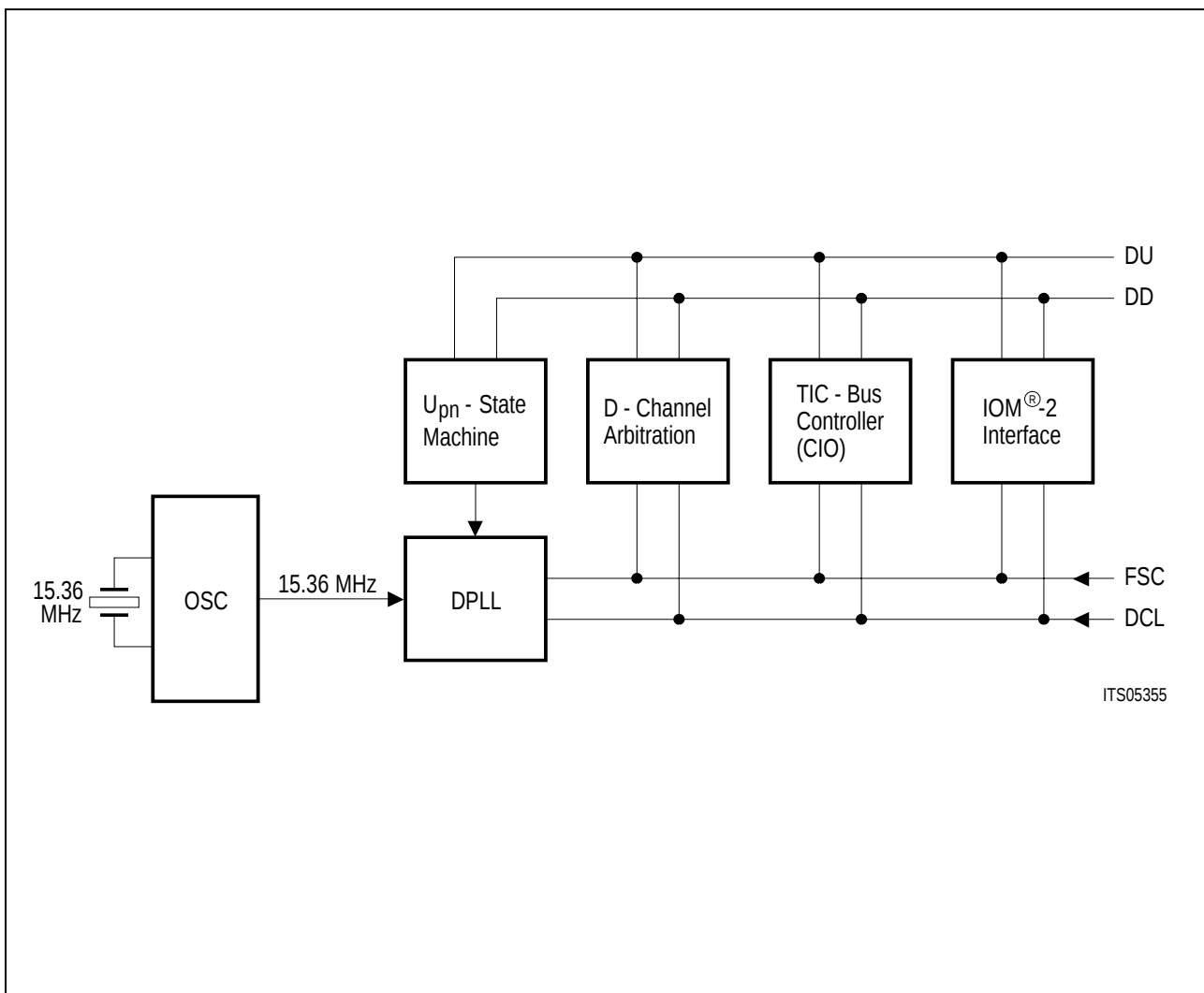
Figure 36 Clock Generation in TR-Mode
