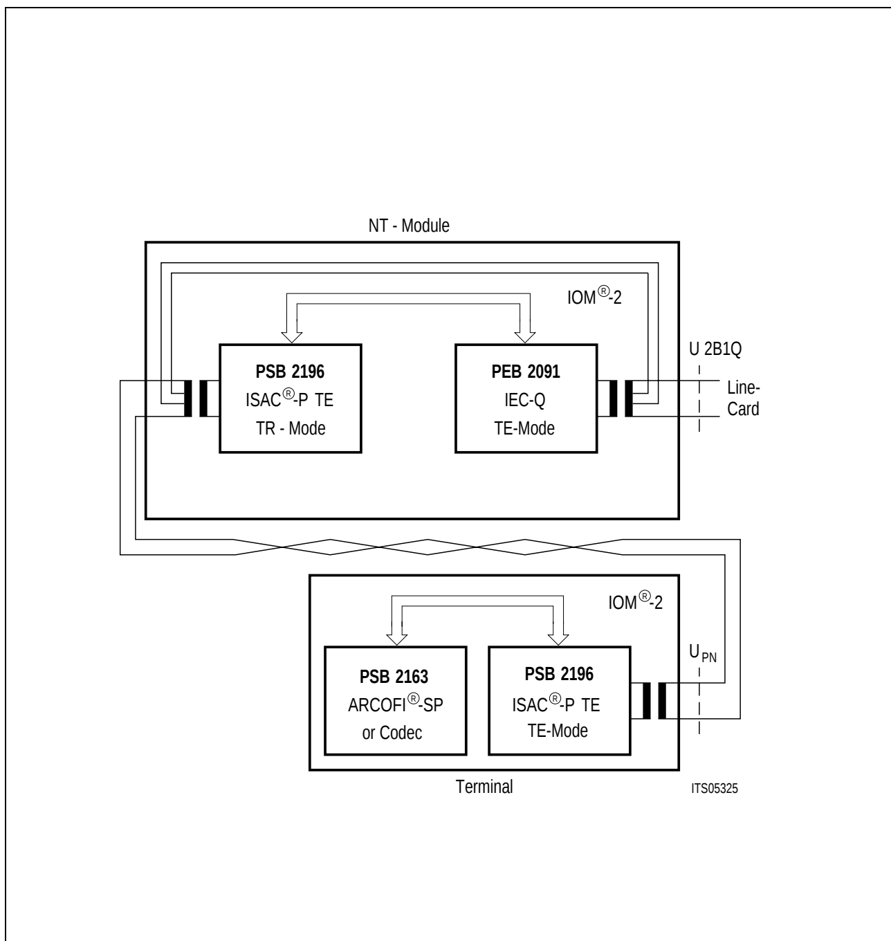
Figure 8 Network Termination Using the ISAC ® -P TE
