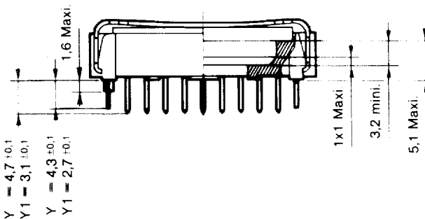
Dip solder
