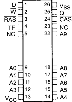
DJ and DN Packages† (Top View)
