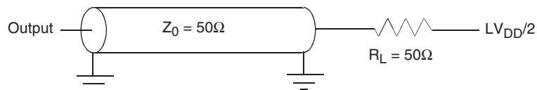
Figure 8-4. eTSEC AC Test Load
