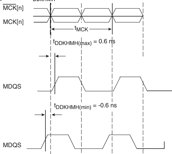
Figure 6-1. Timing Diagram for t_{DDKHMH}
