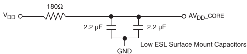
Figure 22-2. PLL Power Supply Filter Circuit with CORE Pins
