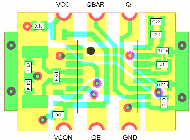
2X Layout (TSSOP)
