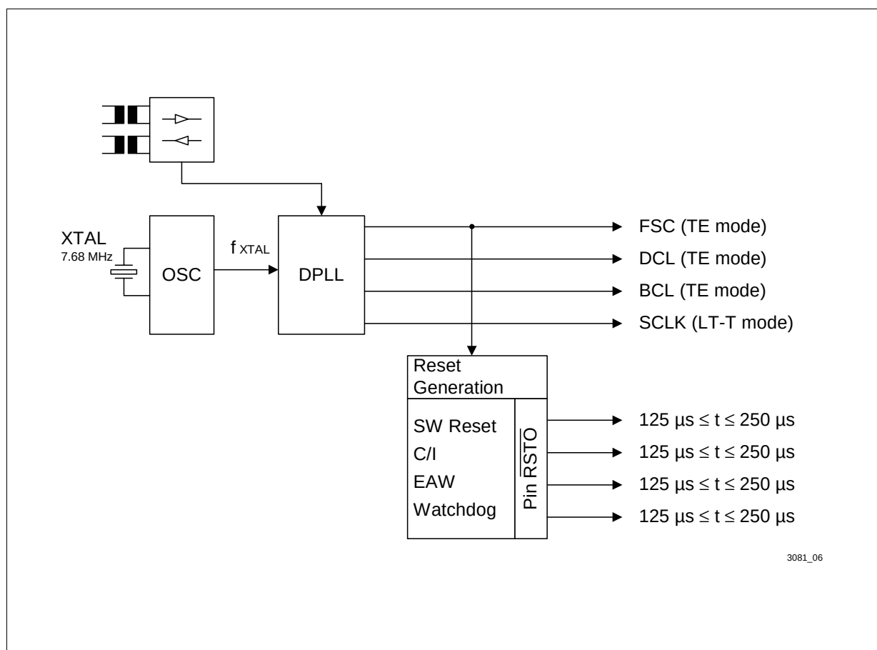
Figure 28 Clock System of the SBCX-X
