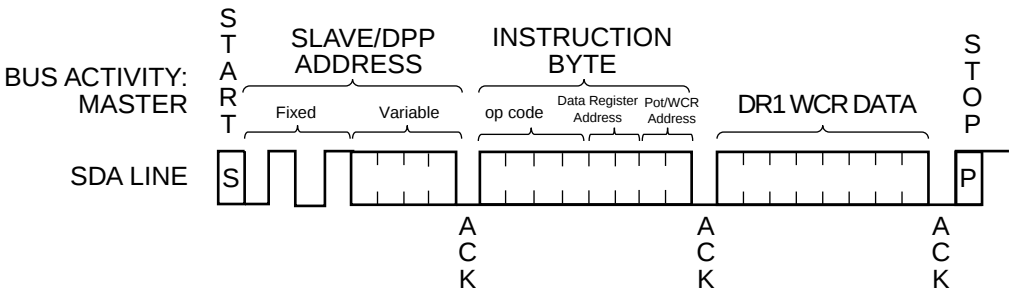
Figure 6. Write Timing
