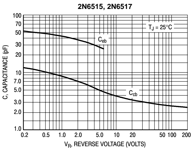
Figure 6. Capacitance
