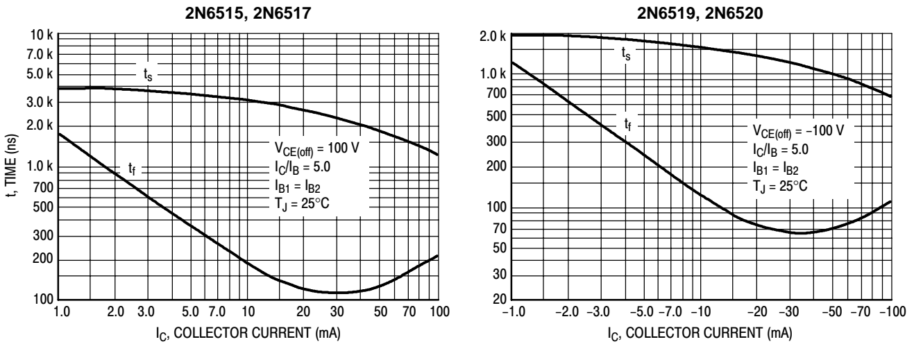
Figure 8. Turn-Off Time
