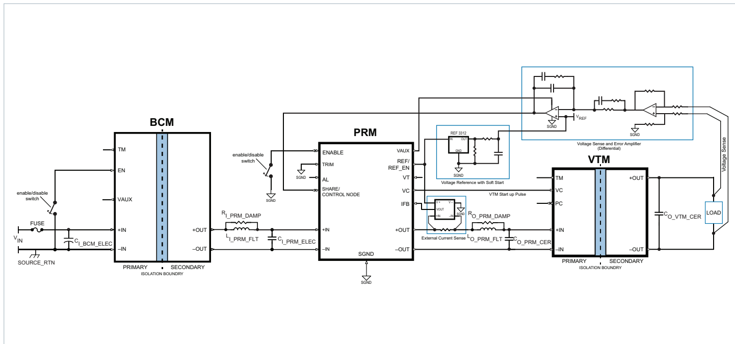
BCM380y475x1K2A30 + PRM + VTM, Remote Sense Configuration
