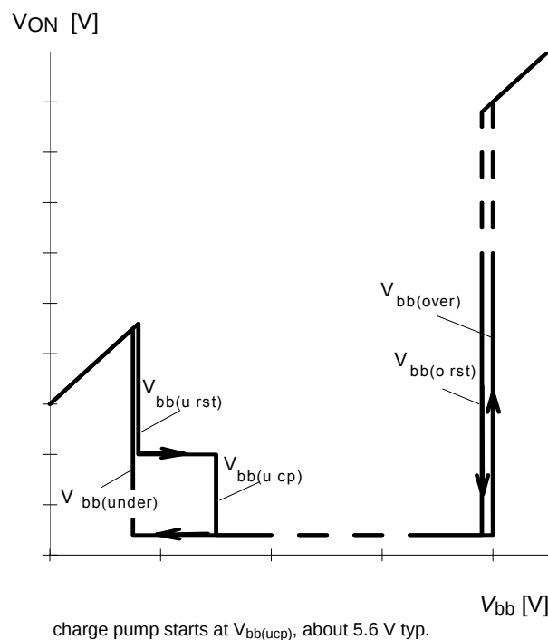
Figure 6: Undervoltage restart of charge pump
