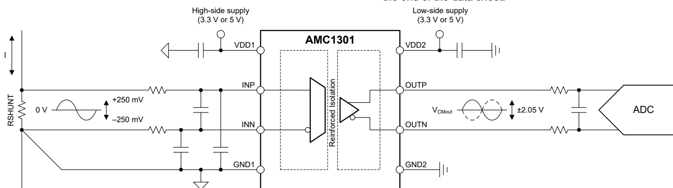
Simplified Schematic
