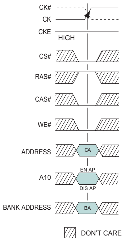
FIGURE 12 – WRITE COMMAND
