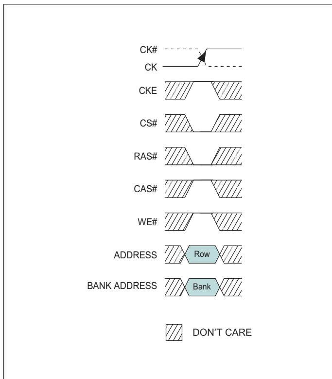
FIGURE 10 – ACTIVE COMMAND
