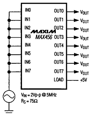
All-Channel Off Isolation (Notes 1, 5-8)
