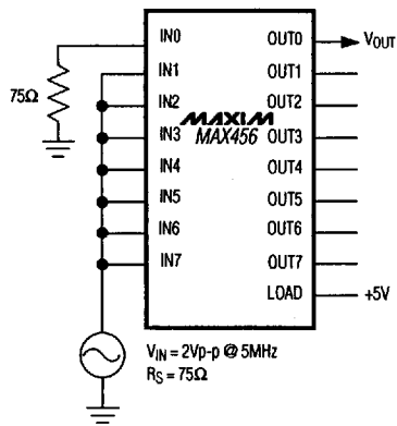
All-Channel Crosstalk (Notes 1, 5, 9, 11, 12)
