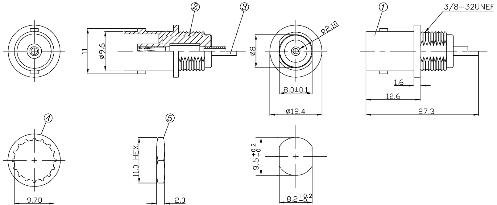
LOCK WASHER
