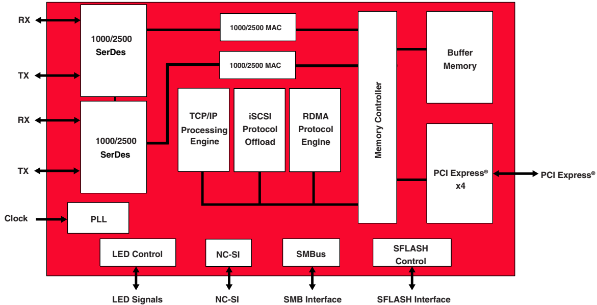
BCM5709S Block Diagram
