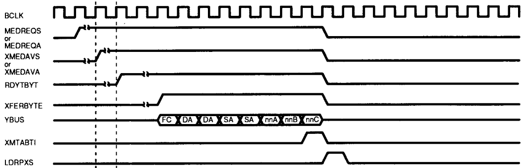
e) XMTABT1 From FORMAC
