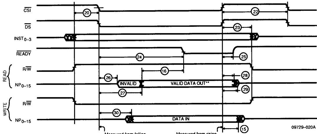
NP-bus Asynchronous Read/Write Timing
