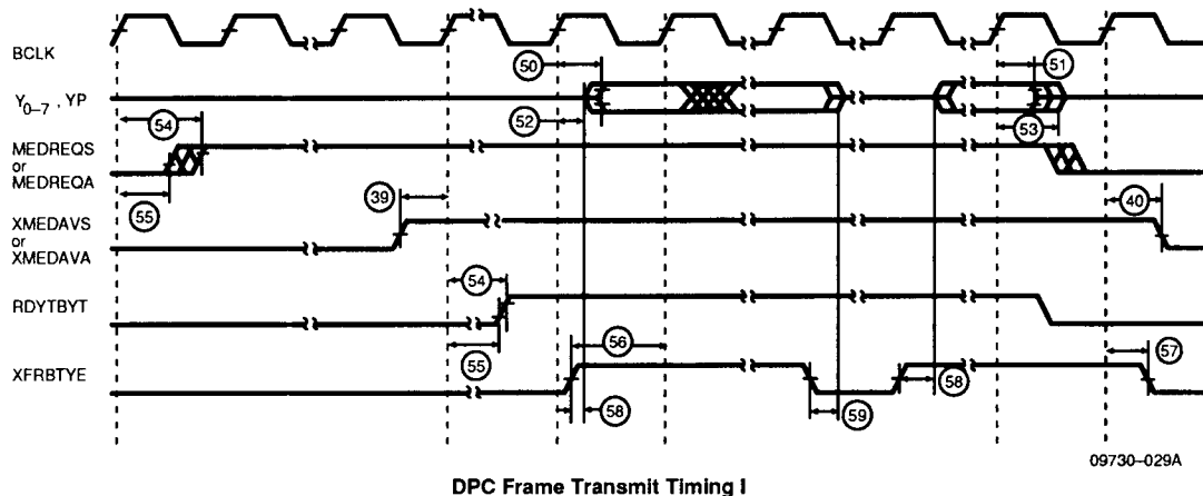
DPC Frame Transmit Timing I
