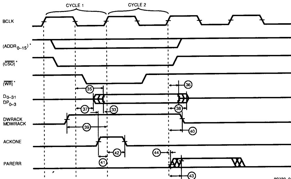
DPC Buffer Memory Write Timing II
