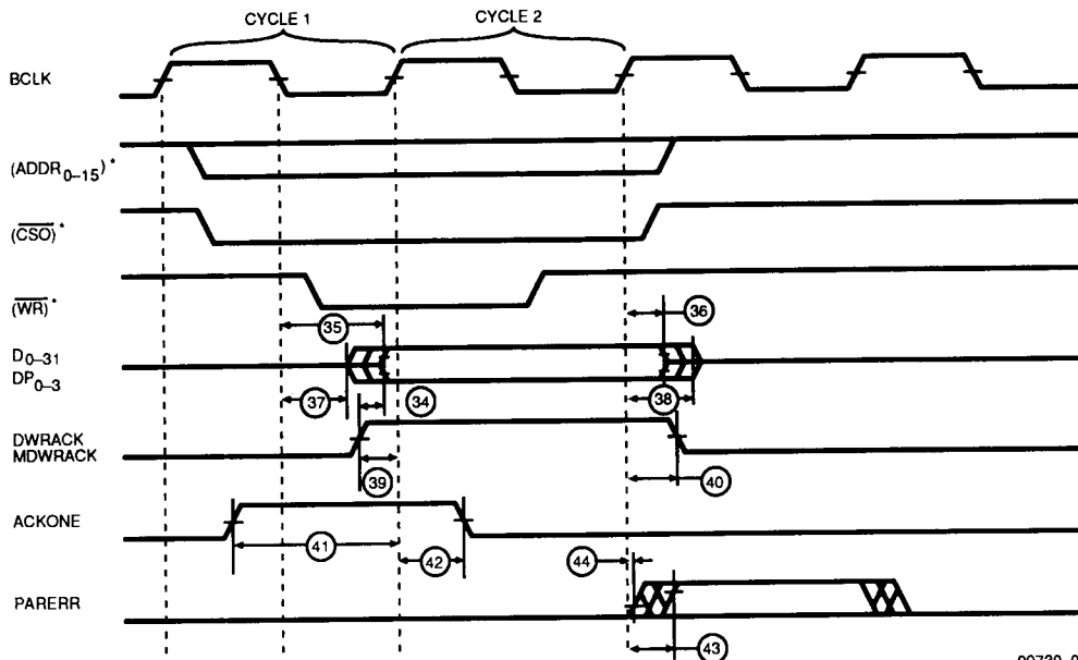
DPC Buffer Memory Write Timing I
