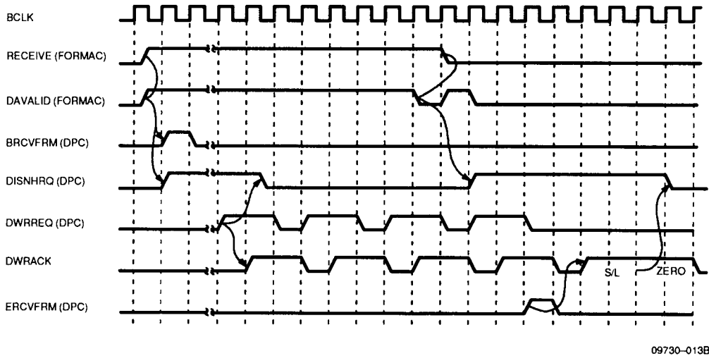
Figure 9. Normal Receive Handshake Between DPC, FORMAC, and RBC
