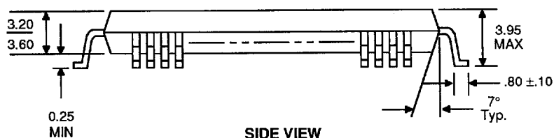
SIDE VIEW
