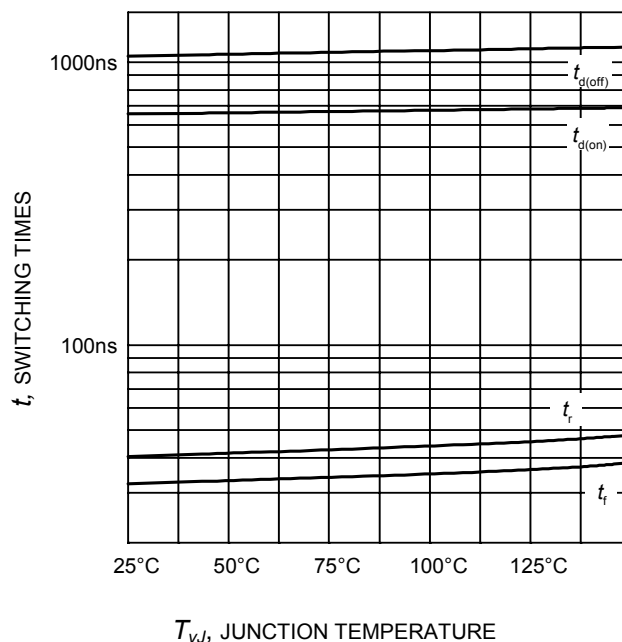
Figure 6. Typical switching times as a function of junction temperature (inductive load, V_{CE} = 300\text{V} , V_{DD} = 15\text{V} , I_C = 15\text{A} Dynamic test circuit in Figure A)
