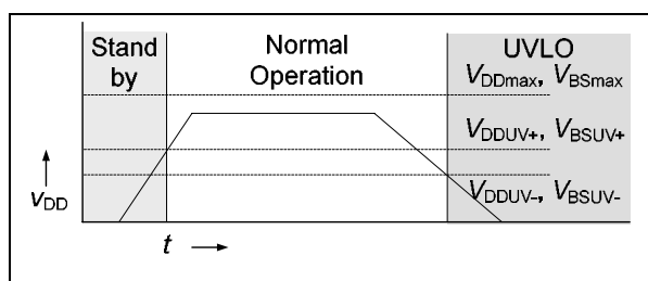
Figure 4: Operating states
