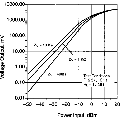
Figure 2. Voltage Output vs. Power Input as a Function of Video Impedance
