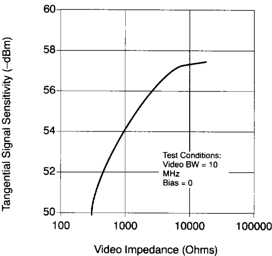
Tangential Signal Sensitivity vs. Video Impedance
